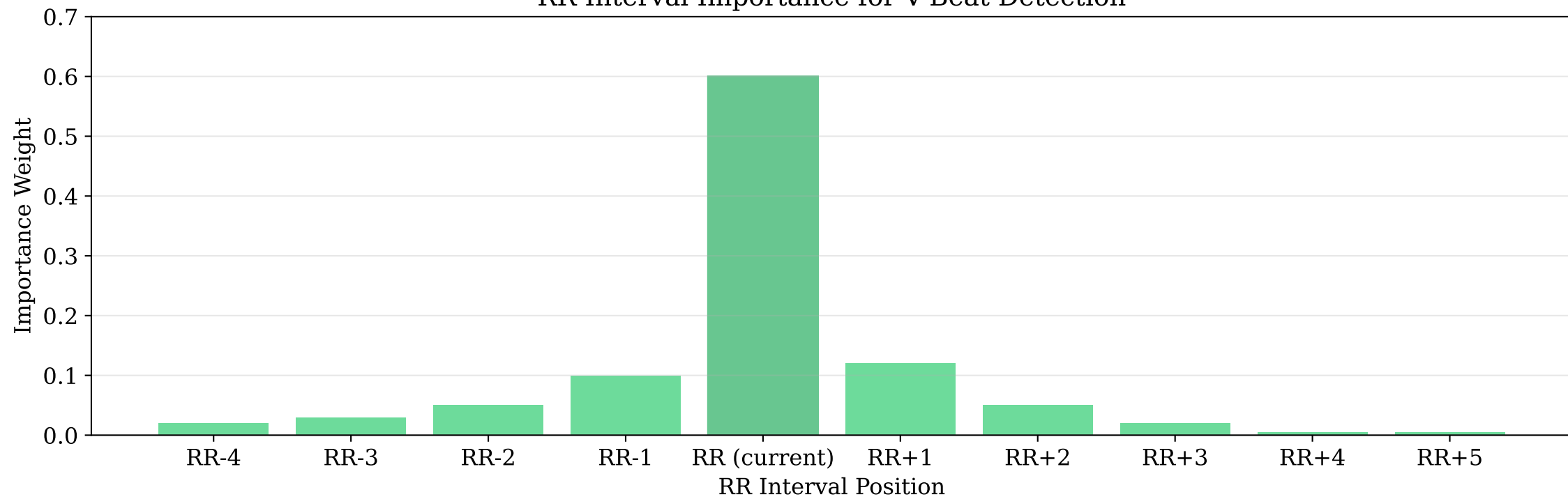
RR Interval Importance for V-Beat Detection
